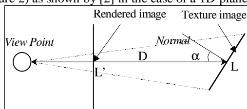
Figure 2: Effect of distance and tilting on rendered image.
