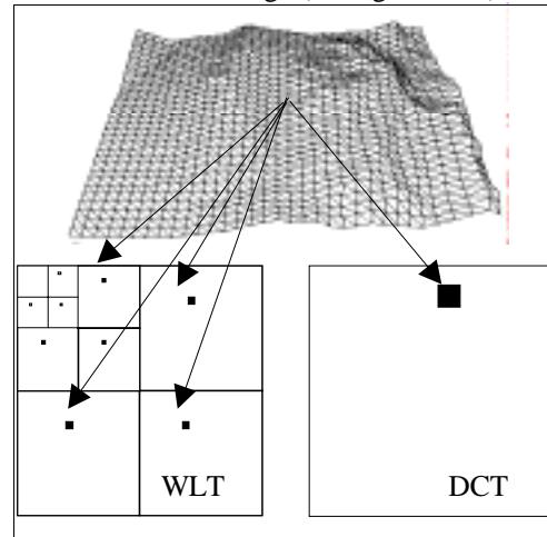
Figure 6: Influence of the position of one grid cell on the coefficients in the frequency domains.
