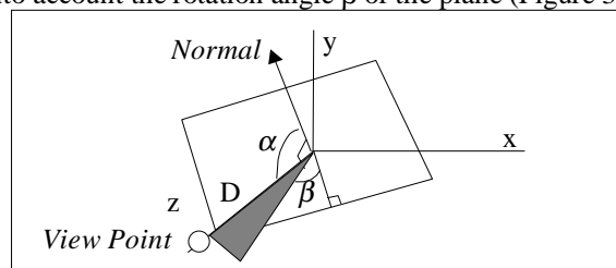
Figure 3: Generalization for a 2D-plane.
